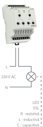
DA3-22M Dimmer universal PWM
